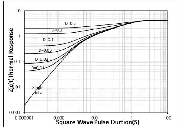
Transient Thermal Response Curve For MS65R600/TO-220MF-K1
