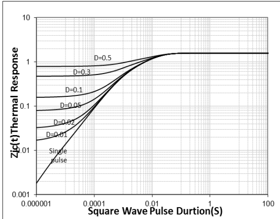
Transient Thermal Response Curve For MS65R600/DPAK
