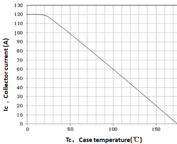
Collector current vs. Case temperature
